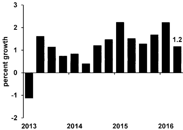
Euro Area GDP Growth
