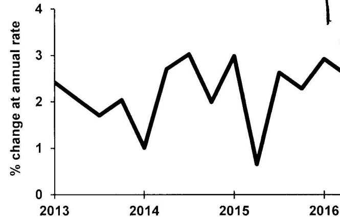
U.S. Wage Inflation
